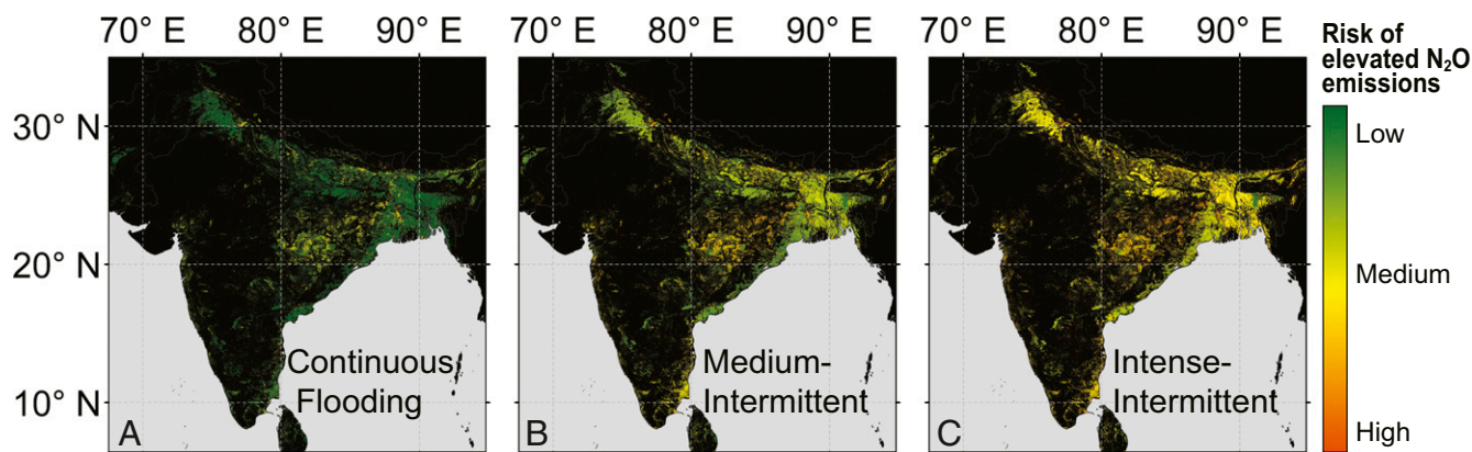
Fig. 2. Qualitative risk of elevated N 2 O emissions from the Indian subcontinent under three flooding scenarios: continuous (A), medium-intermittent (B), and intense-intermittent (C) flooding. The maps depicts rice growing areas in India, Nepal, Pakistan, Sri Lanka, and Bangladesh across 12 water management regimes. For assumed water indices and flooding events, see Dataset S1, Table 38. For a quantitative assessment of emissions, see Dataset S1, Tables 41 and 42.
